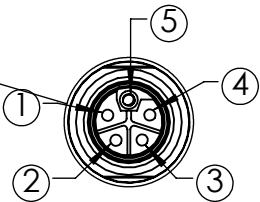
DETAIL B M12L 5 PIN CONNECTOR SCALE 1 : 1
