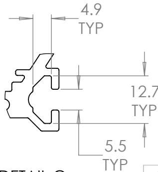
DETAIL C T-SLOT MOUNTING SCALE 1 : 1
