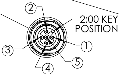
DETAIL A M12A 5 PIN CONNECTOR SCALE 1 : 1
