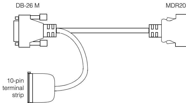
Figure 30. Cable 300-0399
