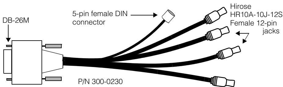
Figure 21. Camera breakout cable with power input, P/N 300-0230
