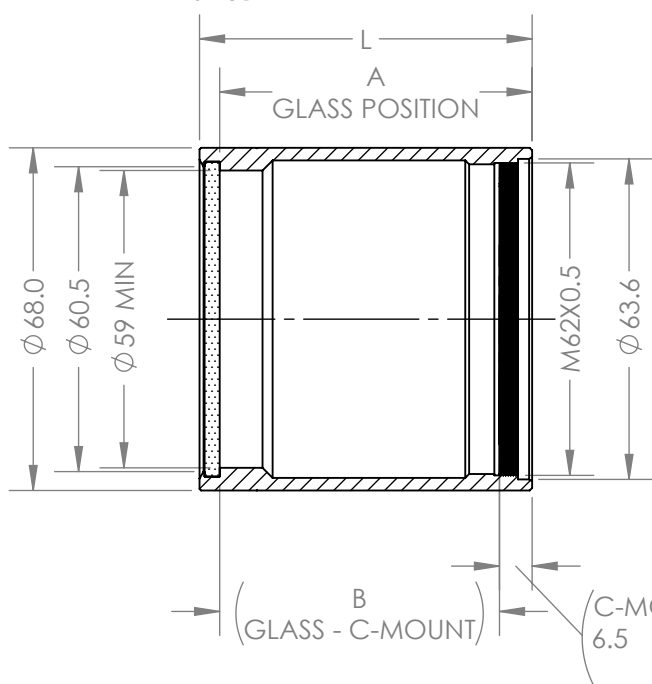
LENS TUBE
