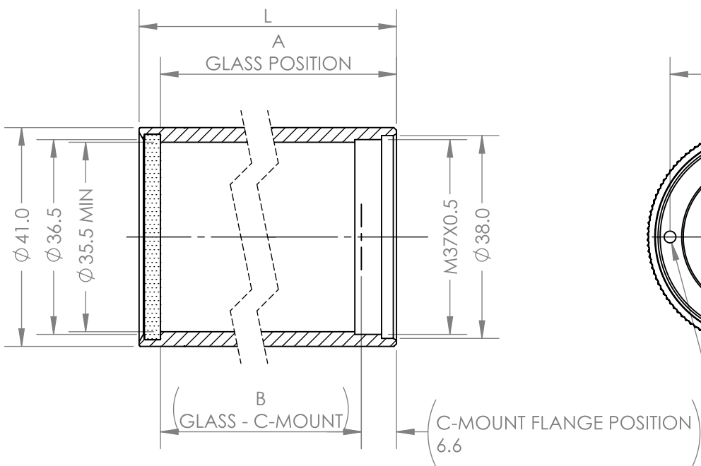
LENS TUBE
