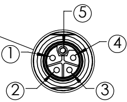
DETAIL B M12L 5 PIN CONNECTOR SCALE 1 : 1
