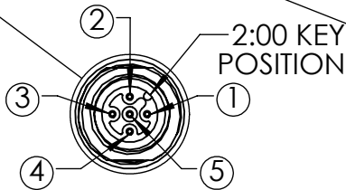
DETAIL A M12A 5 PIN CONNECTOR SCALE 1 : 1
