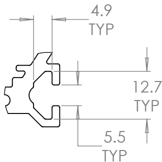
DETAIL C T-SLOT MOUNTING SCALE 1 : 1
