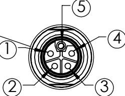
DETAIL B M12L 5 PIN CONNECTOR SCALE 1 : 1
