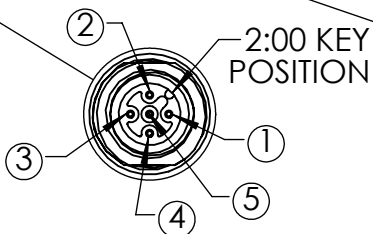
DETAIL A M12A 5 PIN CONNECTOR SCALE 1 : 1
