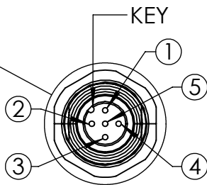
DETAIL B M12 5 PIN CONNECTOR SCALE 1 : 1
