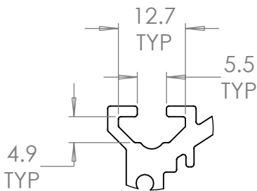
DETAIL A T-SLOT MOUNTING SCALE 1 : 1
