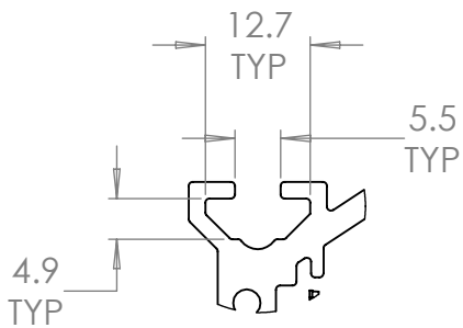
DETAIL A T-SLOT MOUNTING SCALE 1 : 1
