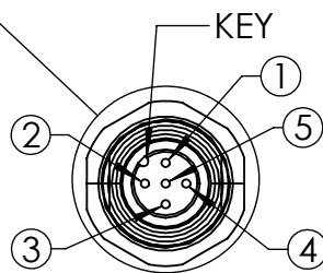
DETAIL B M12 5 PIN CONNECTOR SCALE 1 : 1
