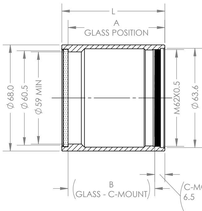
LENS TUBE
