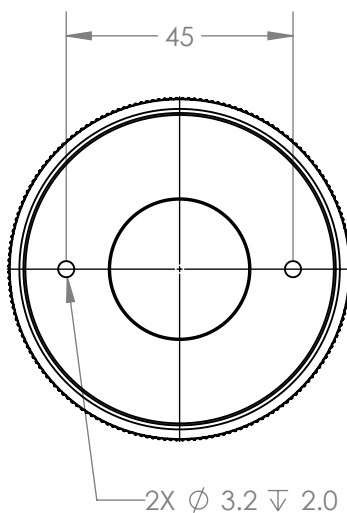
ADAPTER RING
