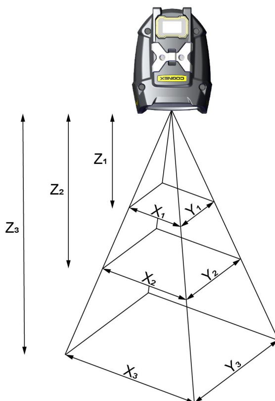
DM8700 HD Field of View Values
