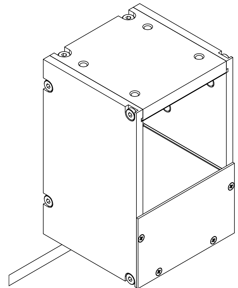
Perspective View
