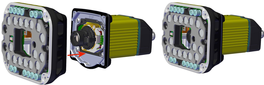
M3 x 6.35 mm captive screws
