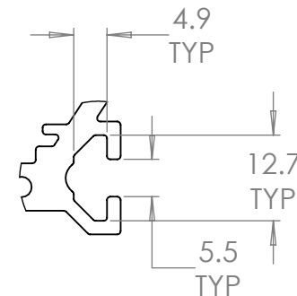
DETAIL C T-SLOT MOUNTING SCALE 1 : 1
