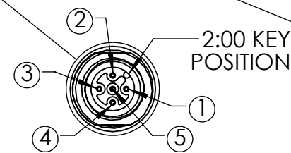
DETAIL A M12A 5 PIN CONNECTOR SCALE 1 : 1
