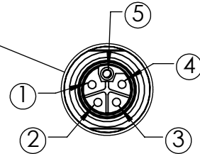
DETAIL B M12L 5 PIN CONNECTOR SCALE 1 : 1
