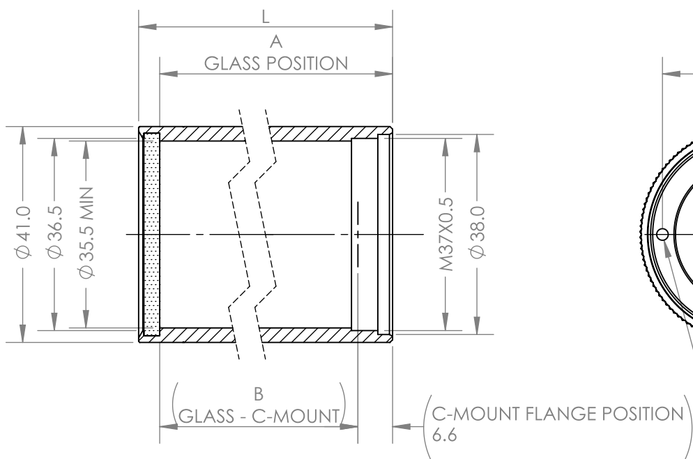
LENS TUBE
